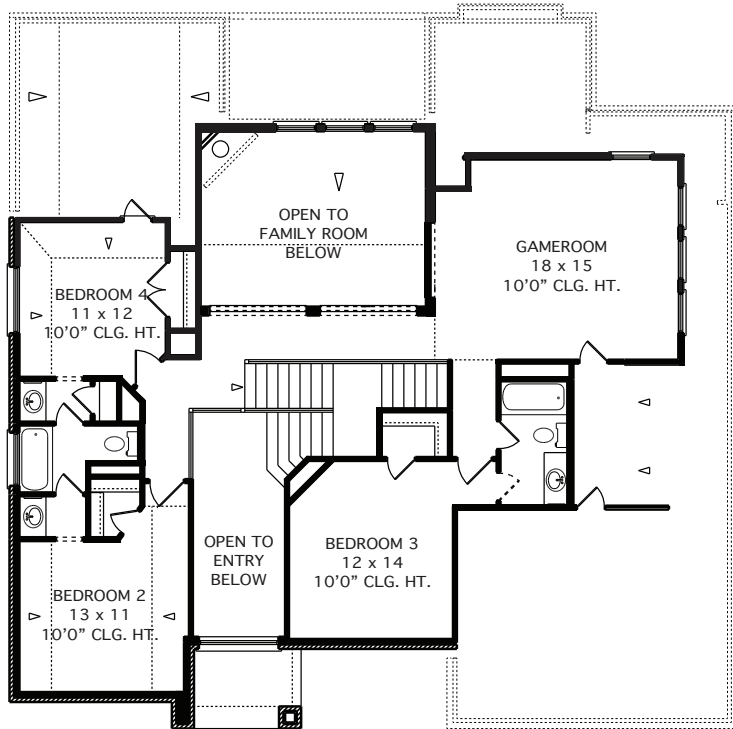
SECOND FLOOR
