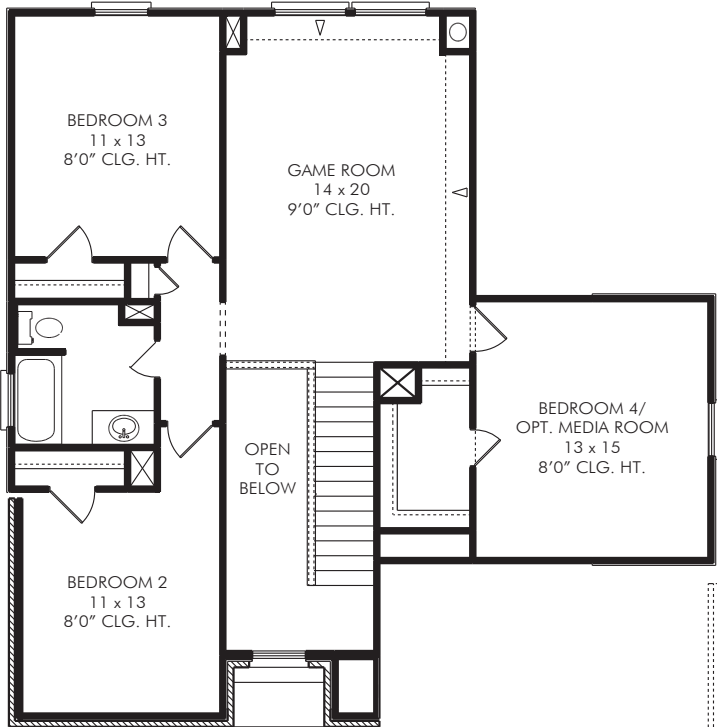
SECOND FLOOR
